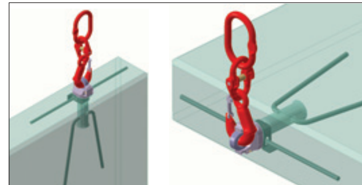
Semplice staffatura Simple reinforcement
